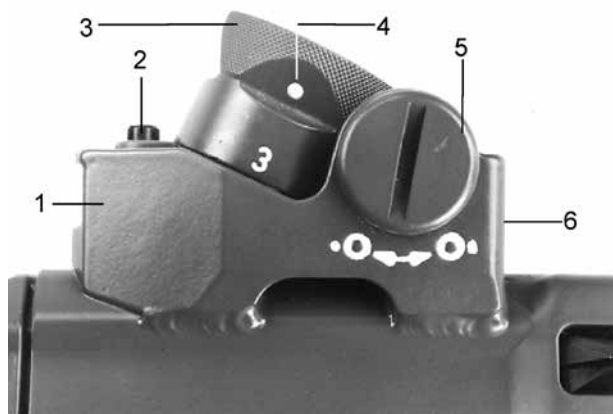
Figure 7: Hausse
