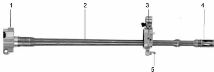
Figure 2 : Canon
